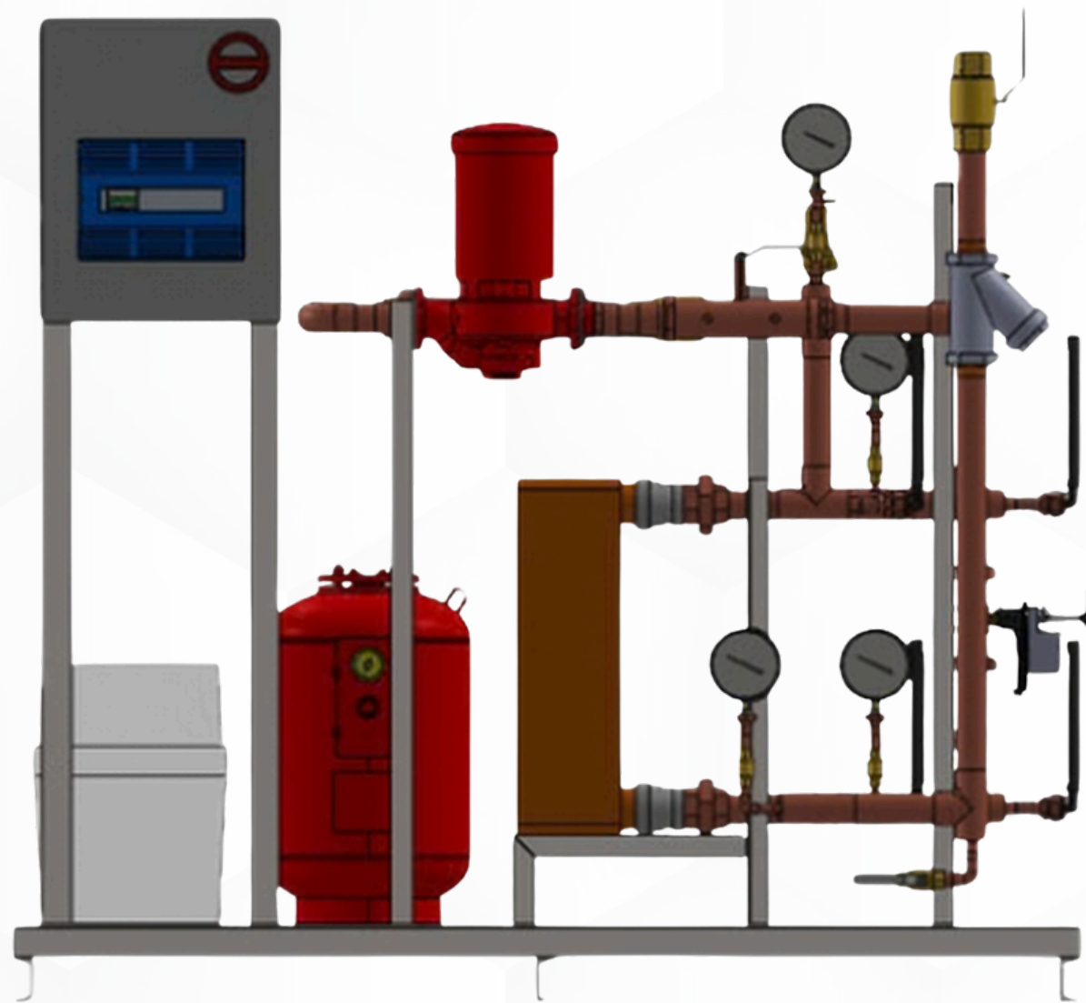
FRONT VIEW
