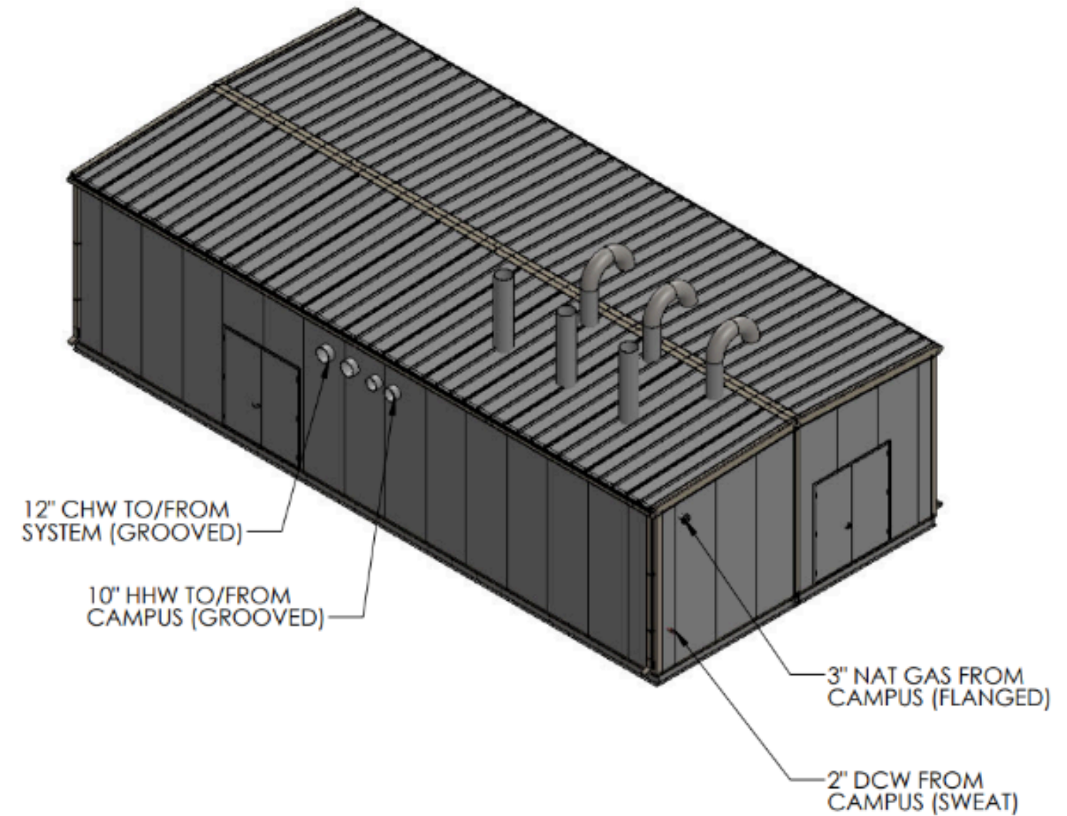
ISOMETRIC VIEW
