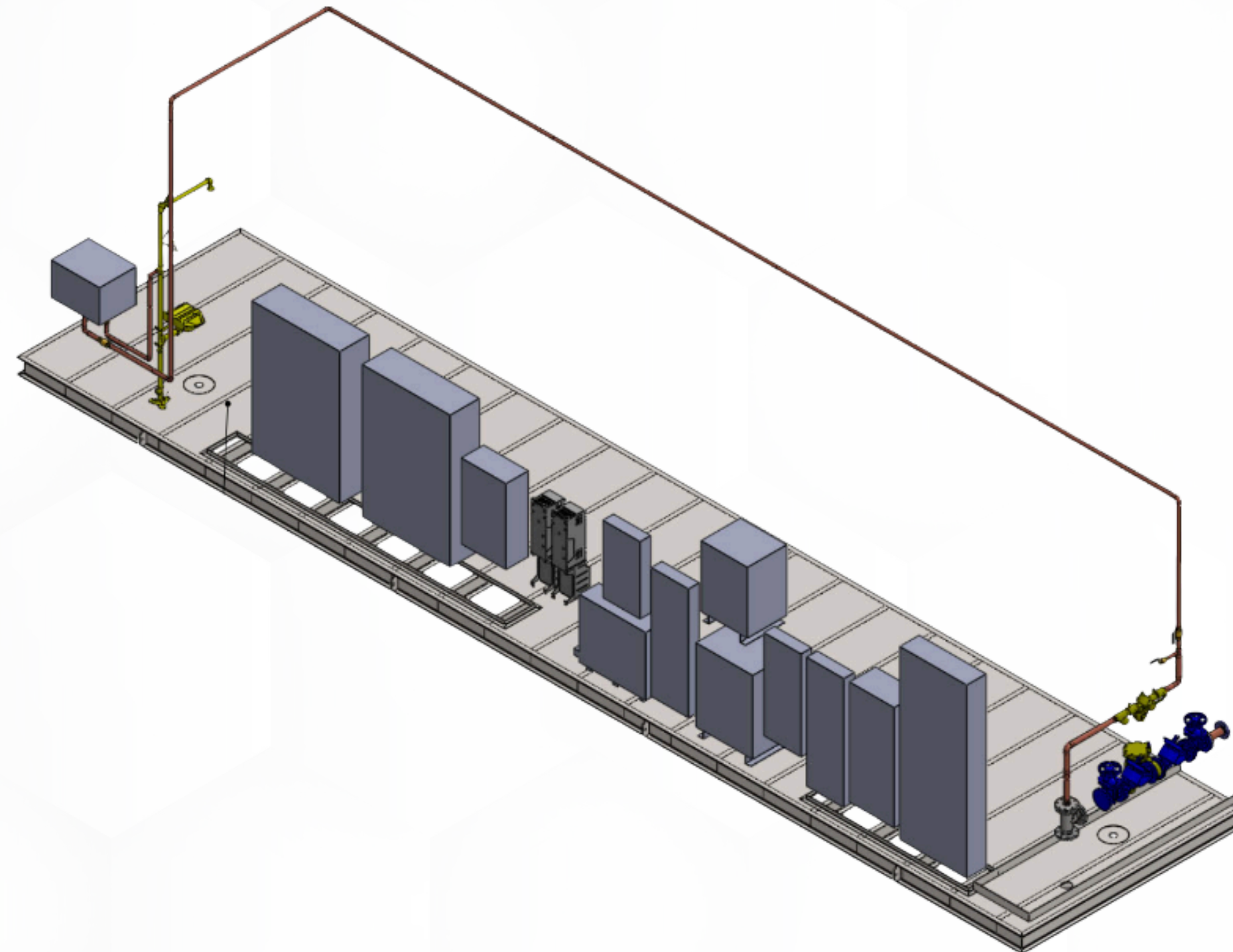
ISOMETRIC VIEW
