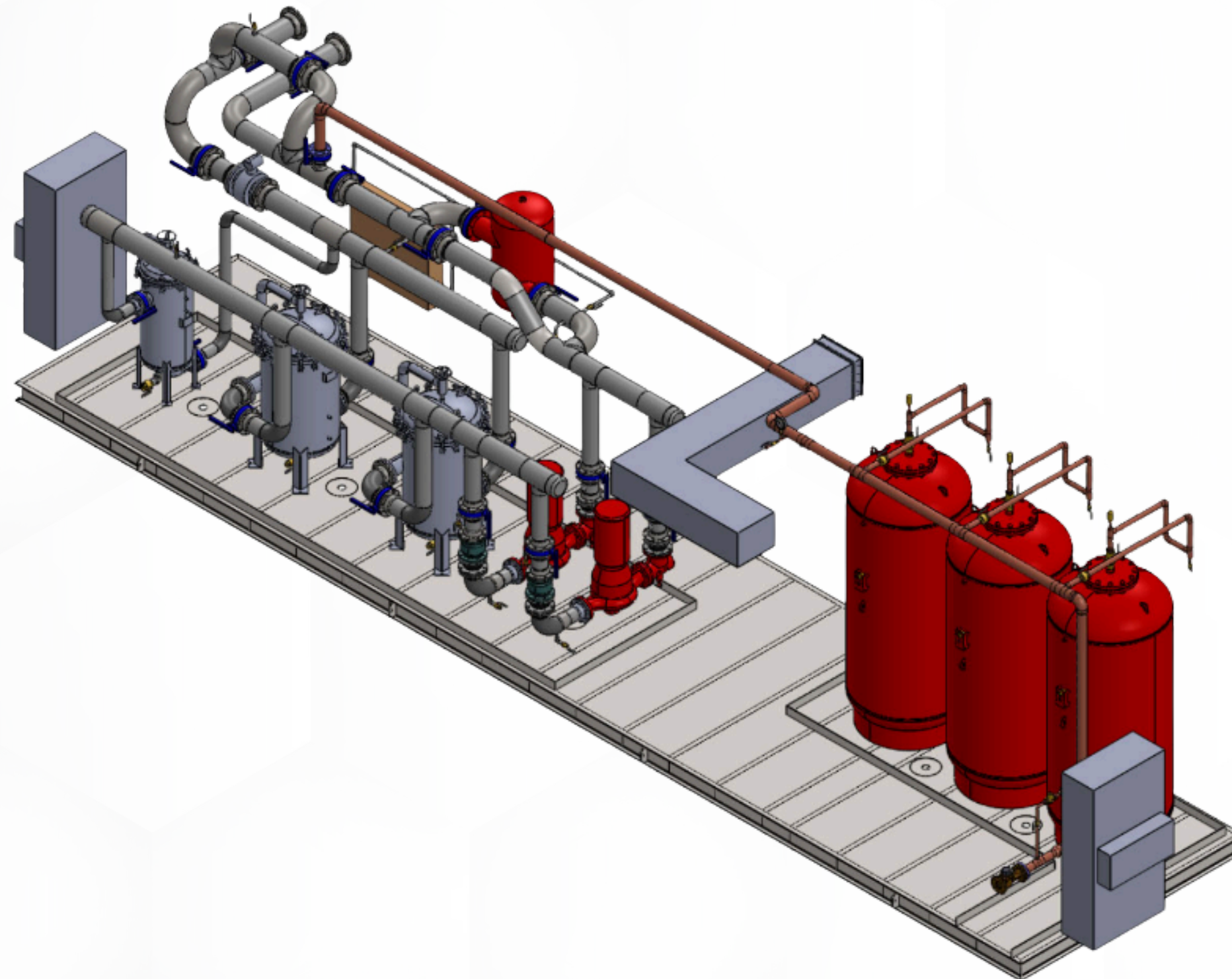
ISOMETRIC VIEW
